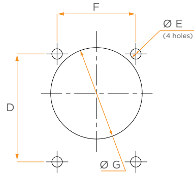
Front Mounting
